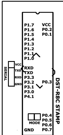
Gambar 1 Tata Letak Port DST-R8C Stamp Perbandingan AT8951 & R8C Stamp
