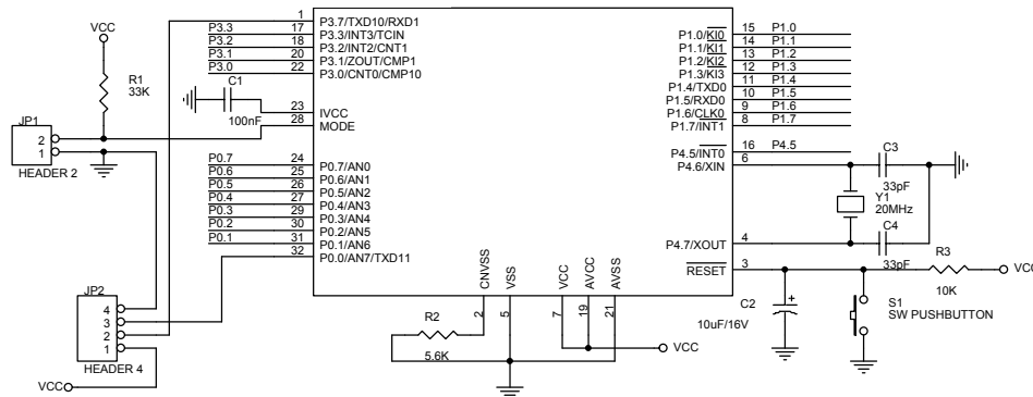
Gambar 1 Tata Letak Port DST-R8C Stamp Perbandingan AT8951 & R8C Stamp
